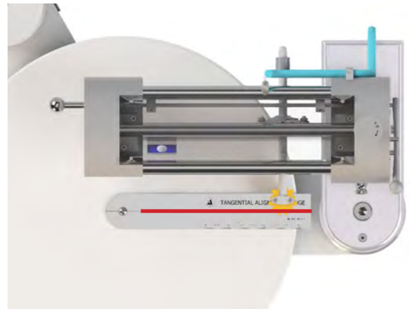
Pic. 22a: Adjustment of the linear tracking
