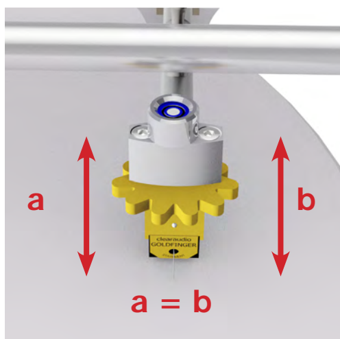
Pic. 26: Azimuth adjustment
